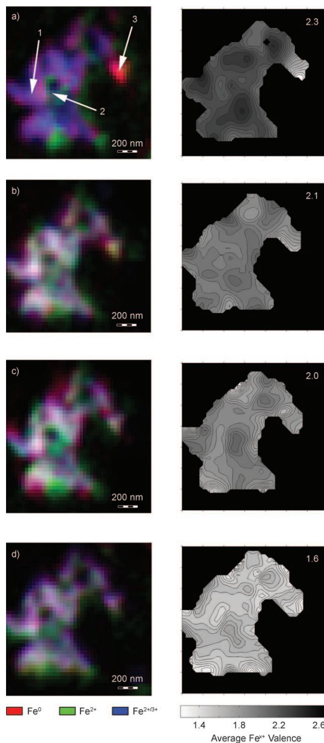
Figure 3. Chemical component images of the catalyst particle, showing the spatial distribution of the different iron species (left) and average valence contour maps (right) in 1 bar H 2 at a) 250 °C, b) 300 °C, c) 350 °C and d) 450 °C. The pixel dimensions (left column) are 35 \times 35 \text{ nm}^2 . The three defined regions are indicated in (a). The average valence of the whole catalyst particle is indicated in the top right corner of the contour maps.
